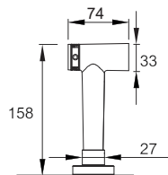
Modern Pull-Out Spray Ref. MP10CP Chrome £105 Ref. MP10BN Brushed Nickel £120 Ref. MP10BB Brushed Brass £130 Ref. MP10MB Matt Black £125 Ref. MP10SS Stainless Steel £125 Min Pressure 0.7 Bar Mounting Hole Size Ø35mm
