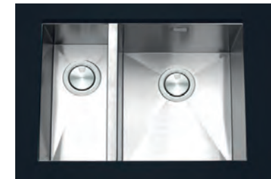
Stark 1.5 bowl Ref. SK55 £500 Overall size: 580/430 mm Main bowl: 340/400/200 mm Half bowl: 180/400/140 mm Min cabinet size: 600 mm
