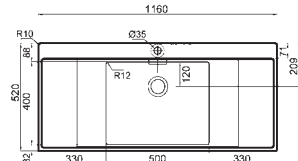
Xeron B50 Single bowl and double drainer Ref. MO1F443A2 £800 Overall size: 1160/520 mm Bowl size: 500/400/200 mm Cutout size: 1142/502 mm Minimum cabinet size: 600 mm Waste included: 90 mm BSW
