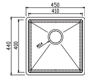
Jazz Single bowl Ref. JA012 £274 Overall size: 450/440 mm Bowl size: 410/400/190 mm Min cabinet size: 450 mm
