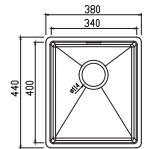
Jazz Single bowl Ref. JA014 £248 Overall size: 380/440 mm Bowl size: 340/400/190 mm Min cabinet size: 400 mm
