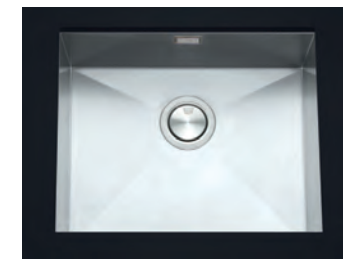
Stark Single bowl Ref. SK50 £400 Overall size: 540/440 mm Bowl size: 500/400/200 mm Minimum cabinet size: 600 mm
