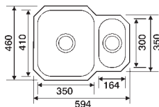
Tango 1.5 bowl Ref. SP20 £260 Overall size: 594/460 mm Bowl size: 350/410/185 mm Half bowl: 164/300 mm Minimum cabinet size: 600 mm
