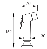
Traditional Pull-Out Spray Ref. TP10CP Chrome £115 Ref. TP10BN Brushed Nickel £130 Ref. TP10BB Brushed Brass £140 Ref. TP10BC Brushed Copper £135 Ref. TP10BZ Brushed Bronze £145 Min Pressure 0.7 Bar Mounting Hole Size Ø35mm
