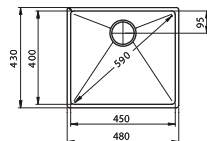
Stereo Single bowl Ref. STE45 £380 Overall size: 480/430 mm Bowl size: 450/400/200 mm Minimum cabinet size: 500 mm
