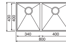
Stark Double bowl Ref. SK77 £776 Overall size: 430/800 mm Left bowl: 340/400/200 mm Right bowl: 400/400/200 mm Minimum cabinet size: 1000 mm
