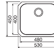
Tango Single bowl Ref. SP480 £240 Overall size: 530/450 mm Bowl size: 480/400/195 mm Minimum cabinet size: 600 mm
