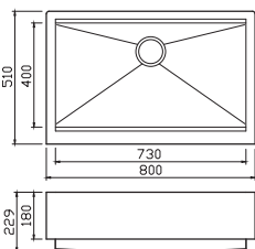
Infinity Smart Single bowl Ref. INS002 £750 Overall size: 800/510 mm Bowl size: 730/400/229 mm Waste included: 90 mm BSW
