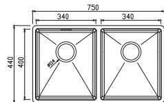
Jazz Double bowl Ref. JA024 £500 Overall size: 750/440 mm Bowl sizes: 340/400/190 mm Minimum cabinet size: 800 mm
