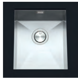
Stark Single bowl Ref. SK34 £315 Overall size: 380/440 mm Bowl size: 340/400/200 mm Minimum cabinet size: 400 mm
