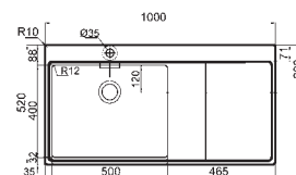
Xeron 105 Large bowl and drainer Ref. ML1F143A2 LHD £693 Ref. ML1F243A2 RHD £693 Overall size: 1000/520 mm Bowl size: 500/400/200 mm Cutout size: 982/502 mm Minimum cabinet size: 600 mm Waste included: 90 mm BSW
