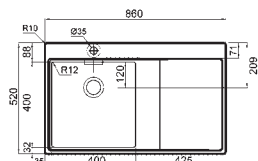
Xeron 86 Single bowl and drainer Ref. MH1F143A2 LHD £633 Ref. MH1F243A2 RHD £633 Overall size: 860/520 mm Bowl size: 400/400/200 mm Cutout size: 842/502 mm Minimum cabinet size: 500 mm Waste included: 90 mm BSW
