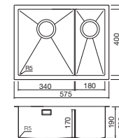
Volta 1.5 bowl Ref. VL53LDBC £655 Ref. VL53RDBC £655 Overall size: 575/450 mm Bowl size: 340/400/190 mm Half bowl: 180/400/190 mm Cutout size: 555/430 mm (Inset) Minimum cabinet size: 600 mm Wastes included: 2 x 90 mm BSW & Plumbing Kit
