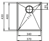
Stereo Single bowl Ref. STE34 £315 Overall size: 370/430 mm Bowl size: 340/400/200 mm Minimum cabinet size: 400 mm
