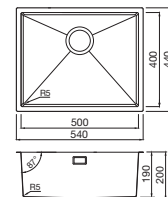
Volta Single bowl Ref. VL500DBC £485 Overall size: 540/440 mm Bowl size: 500/400/190 mm Cutout size: 520/420 mm (Inset) Minimum cabinet size: 600 mm Waste included: 90 mm BSW
