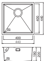
Volta Single bowl Ref. VL400DBB £435 Overall size: 440/440 mm Bowl size: 400/400/190 mm Cutout size: 420/420 mm (Inset) Minimum cabinet size: 500 mm Waste included: 90 mm BSW
