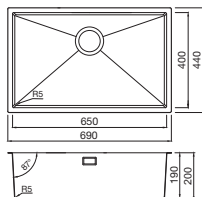
Volta Single bowl Ref. VL650DBB £540 Overall size: 690/440 mm Bowl size: 650/400/190 mm Cutout size: 670/420 mm (Inset) Minimum cabinet size: 800 mm Waste included: 90 mm BSW
