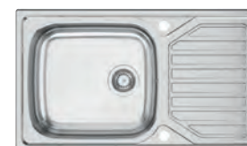
Okio Large bowl and small drainer Ref. OK86L £180 Overall size: 860/500 mm Bowl size: 450/400/160 mm Cutout size: 836/476 mm Minimum cabinet size: 500 mm Waste included: 90 mm BSW
