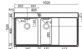
Xeron 100 1.5 bowl and drainer Ref. ML7F148A2 LHD £851 Ref. ML4F128A2 RHD £851 Overall size: 1000/520 mm Bowl size: 340/400/200 mm Half bowl: 170/400/170 mm Cutout size: 982/502 mm Minimum cabinet size: 600 mm Waste included: 2 x 90 mm BSW & Plumbing Kit
