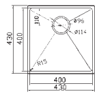
Stereo Single bowl Ref. STE40 £360 Overall size: 430/430 mm Bowl size: 400/400/200 mm Minimum cabinet size: 500 mm
