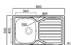
Okio Single bowl and drainer Ref. 7507123 £180 Overall size: 860/500 mm Bowl size: 340/400/160 mm Cutout size: 836/476 mm Minimum cabinet size: 450 mm Waste included: 90 mm BSW
