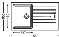
Tivoli Single bowl and drainer Ref. TIV D100S £289 Overall size: 860/500 mm Bowl size: 347/430/200 mm Cutout size: 840/480 mm Minimum cabinet size: 450 mm Standard waste kit included
