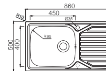
Okio Large bowl and small drainer Ref. OK86L £180 Overall size: 860/500 mm Bowl size: 450/400/160 mm Cutout size: 836/476 mm Minimum cabinet size: 500 mm Waste included: 90 mm BSW
