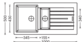
Tivoli 1.5 bowl and drainer Ref. TIV D150 £299 Overall size: 1000/500 mm Bowl size: 345/430/200 mm Half bowl: 155/340/146 mm Cutout size: 980/480 mm Minimum cabinet size: 600 mm Standard waste kit included
