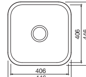
Tango Single bowl Ref. SP400 £180 Overall size: 446/440 mm Bowl size: 406/406/180 mm Minimum cabinet size: 450 mm
