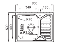
Okio Small bowl & drainer Ref. 7510223 £195 Overall size: 650/500 mm Cutout size: 630/480 mm Bowl depth: 160 mm Minimum cabinet size: 450 mm Waste included: 90mm BSW
