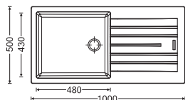
Tivoli Large bowl and drainer Ref. TIV D100L £299 Overall size: 1000/500 mm Bowl size: 480/430/200 mm Cutout size: 980/480 mm Minimum cabinet size: 600 mm Standard waste kit included
