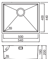
Volta Single bowl Ref. VL500DBB £485 Overall size: 540/440 mm Bowl size: 500/400/190 mm Cutout size: 520/420 mm (Inset) Minimum cabinet size: 600 mm Waste included: 90 mm BSW
