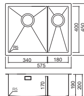
Volta 1.5 bowl Ref. VL53LDBC LH Main Bowl £655 Ref. VL53RDBC RH Main Bowl £655 Overall size: 575/450 mm Bowl size: 340/400/190 mm Half bowl: 180/400/190 mm Cutout size: 555/430 mm (Inset) Minimum cabinet size: 600 mm Wastes included: 2 x 90 mm BSW & Plumbing Kit
