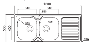
Okio Double bowl and drainer Ref. 7510823 £303 Overall size: 1200/500 mm Bowl sizes : 340/400/160 mm Cutout size: 1176/476 mm Minimum cabinet size: 800 mm Waste included: 2 x 90 mm BSW & Plumbing Kit
