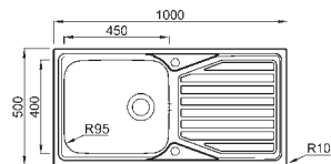
Okio Large bowl and drainer Ref. 7510723 £228 Overall size: 1000/500 mm Bowl size: 450/400/160 mm Cutout size: 976/476 mm Minimum cabinet size: 500 mm Waste included: 90 mm BSW
