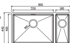
Jazz 1.5 bowl Ref. JA022LH LH Main Bowl £500 Ref. JA022RH RH Main Bowl £500 Overall size: 800/440 mm Bowl size: 550/400/190 mm Half bowl: 180/400/125 mm Minimum cabinet size: 800 mm
