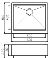
Infinity Smart Single bowl Ref. INS001 £668 Overall size: 600/510 mm Bowl size: 530/400/229 mm Waste included: 90 mm BSW
