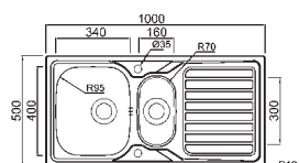
Okio 1.5 bowl and drainer Ref. 7510423 £280 Overall size: 1000/500 mm Bowl size: 340/400/160 mm Half bowl: 160/350/90 mm Cutout size: 976/476 mm Minimum cabinet size: 600 mm Waste included: 2 x 90 mm BSW & Plumbing Kit
