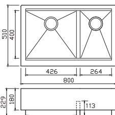
Infinity Smart 1.5 bowl Ref. INS003 £863 Overall size: 800/510 mm Bowl size: 426/400/229 mm Half bowl: 264/400/229 mm Waste included: 2 x 90 mm BSW & Plumbing Kit
